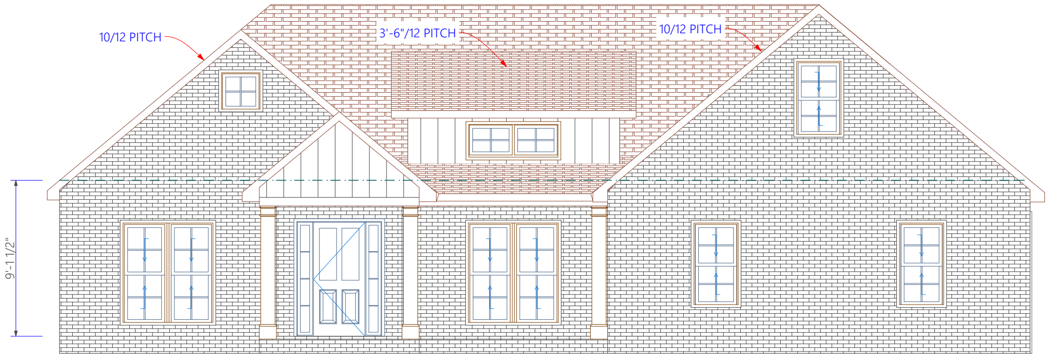
FRONT ELEVATION HIP
