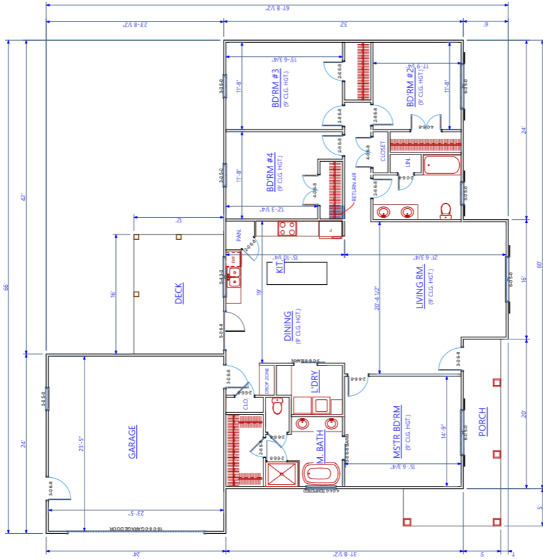
FIRST FLOOR PLAN LIVING AREA = 2,016 SQ. FT. GARAGE = 576 SQ. FT.
